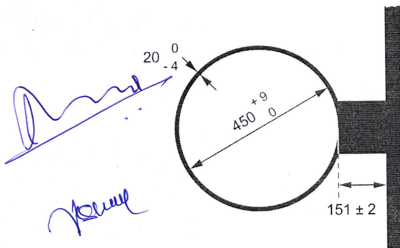
Diagram 4 Basket ring dimensions
